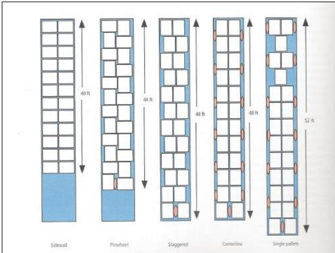
Figure 1: Courtesy of University of California Refrigerated Trailer Transport of Perishable Foods
