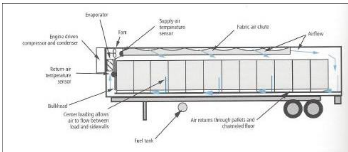
Figure 2: Courtesy of University of California Refrigerated Trailer Transport of Perishable Foods
